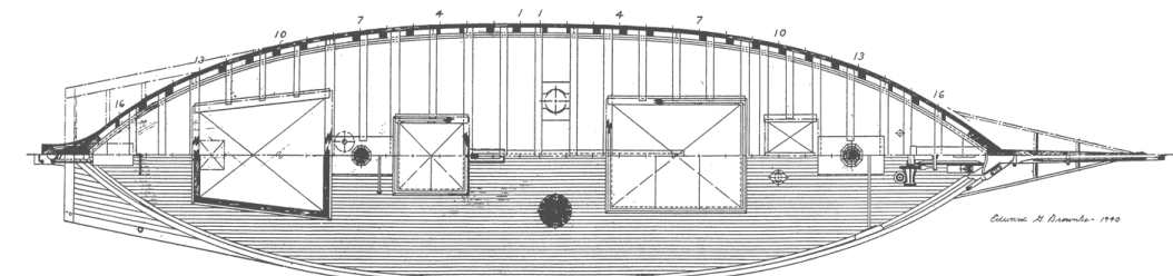
PLATE XVI B. STRUCTURAL PLAN OF FRAME BUGYE Lizzie J. Cox.
