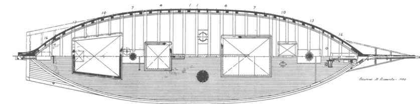
PLATE XVI B. STRUCTURAL PLAN OF FRAME BARGE Lizzie J. Cox.
