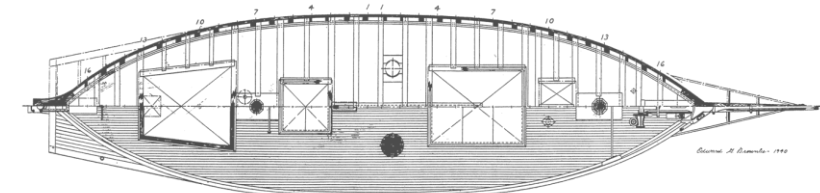
PLATE XVI B. STRUCTURAL PLAN OF FRAME BARGE Lizzie J. Cox.
